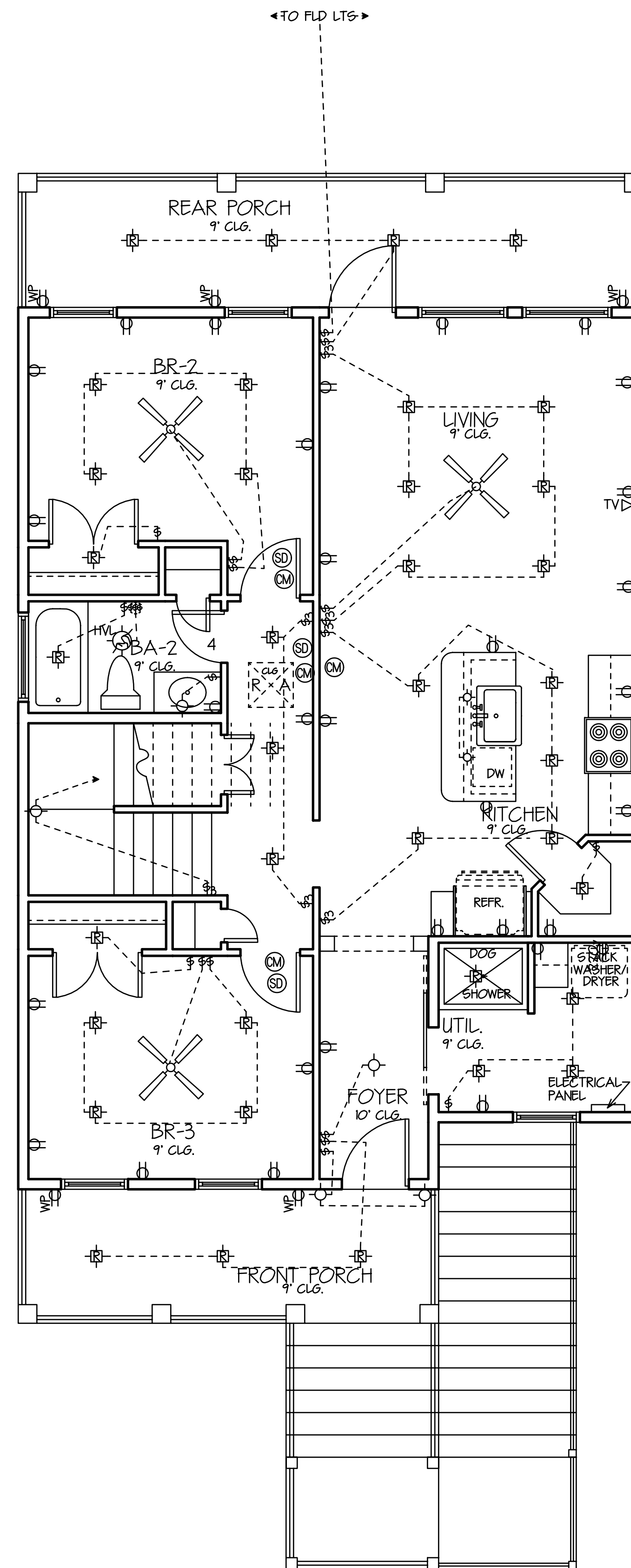
1ST LEVEL ELECTRICAL PLAN SCALE 1/4"=1'-0"
