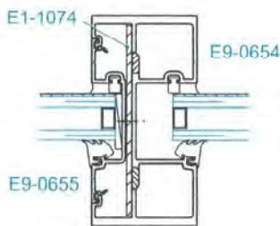
SECTION 5A VERTICAL w/ OPTIONAL STEEL & 1" GLAZING
