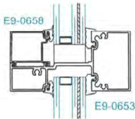
SECTION 2 HORIZONTAL
