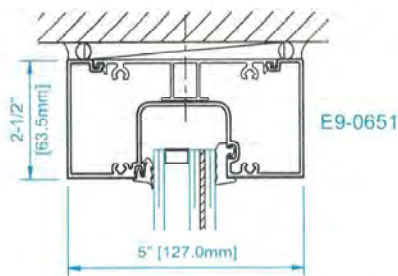
SECTION 1 HEAD
