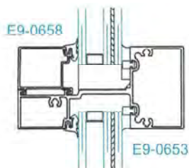
SECTION 2 HORIZONTAL
