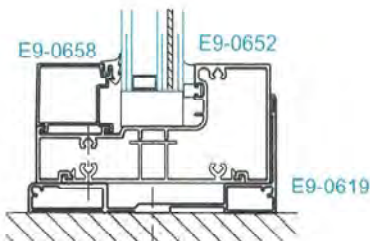
SECTION 3 SILL
