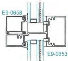
SECTION 2 HORIZONTAL
