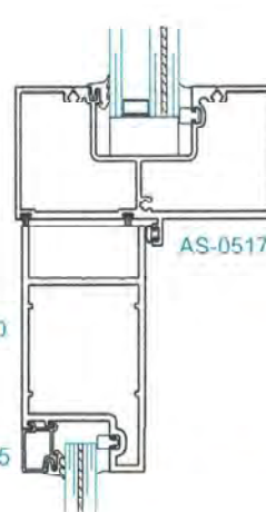
SECTION 8 TRANSOM BAR
