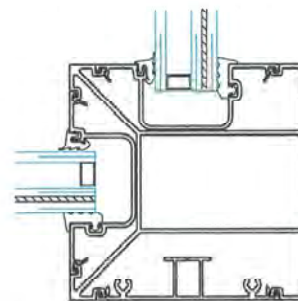
SECTION 6 90° OUTSIDE CORNER
