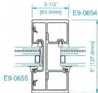
SECTION 5 VERTICAL
