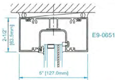
SECTION 1 HEAD
