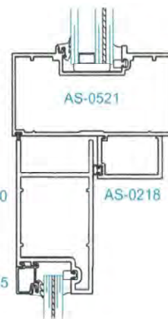
SECTION 8A TRANSOM BAR FOR OHCC
