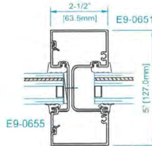
SECTION 5 VERTICAL
