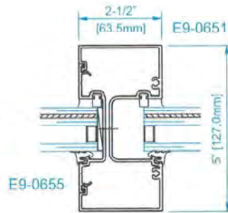
SECTION 5 VERTICAL
