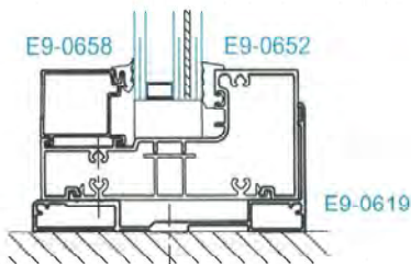
SECTION 3 SILL
