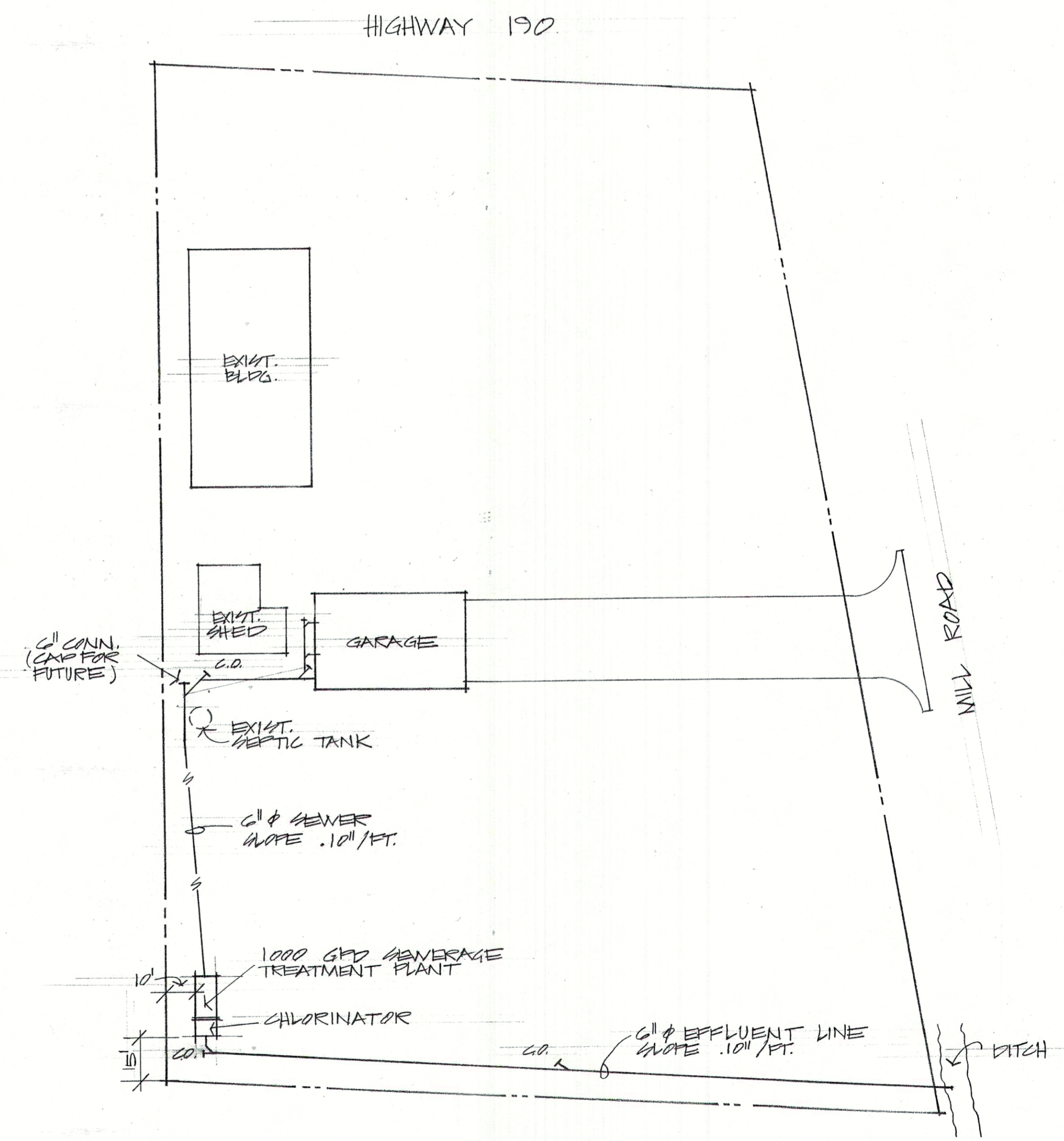
SITE PLAN
