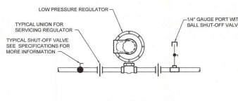
GAS REGULATOR DETAIL N.T.S.
