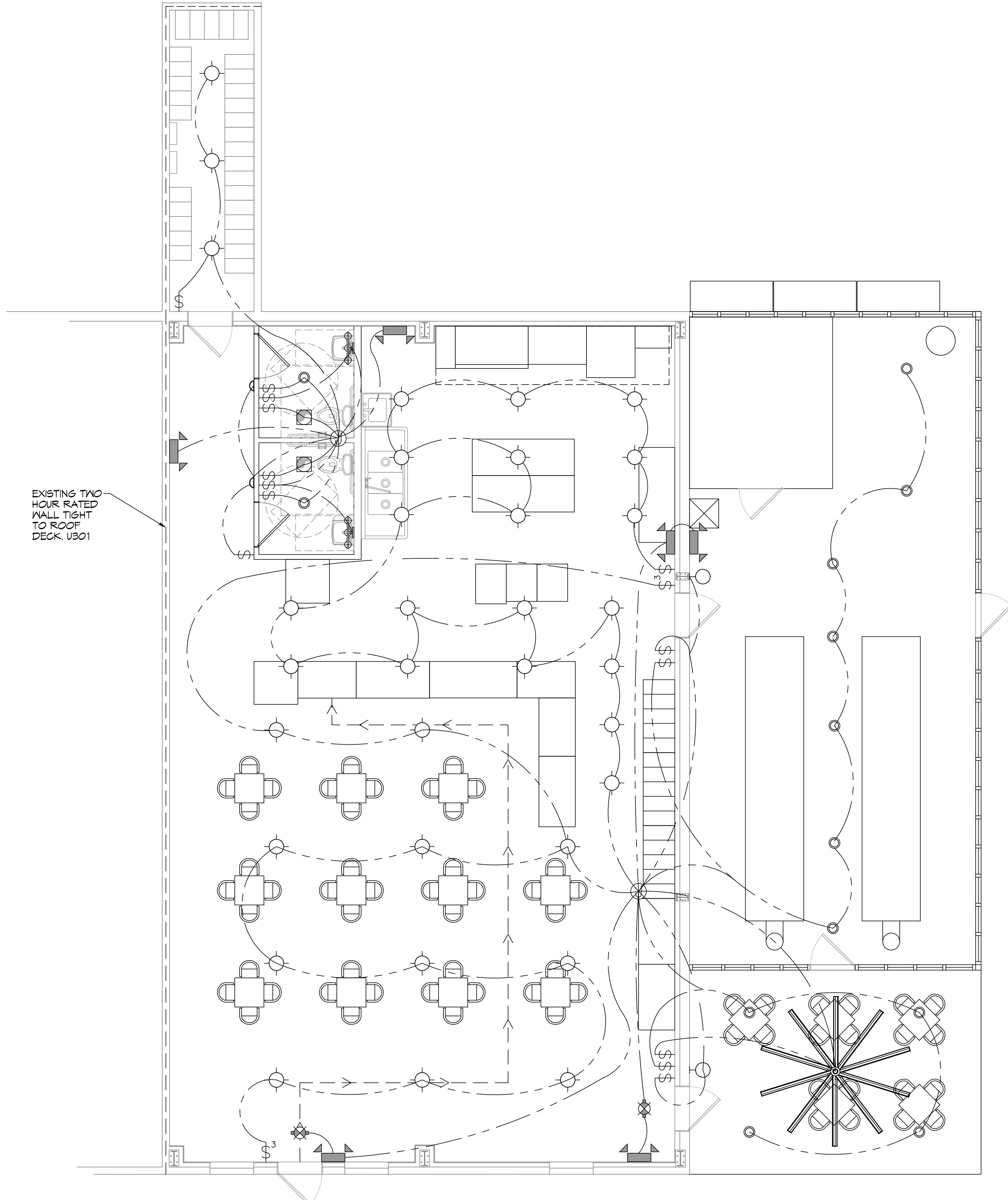
11 LIGHTING PLAN SCALE: 3/32"=1'-0"
