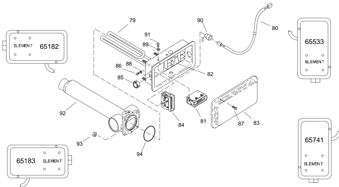
Heater Assy
