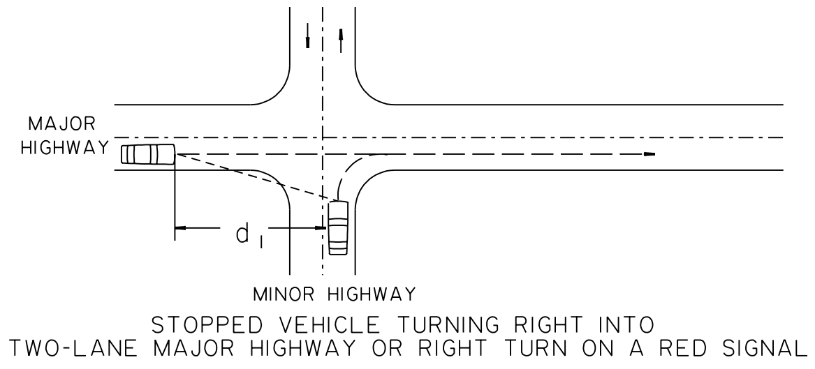
Figure 4-1: Intersection sight distance at at-grade intersections.
