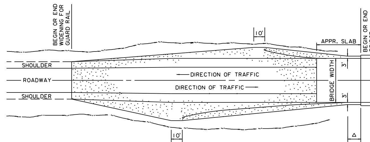
EMBANKMENT WIDENING DETAIL
