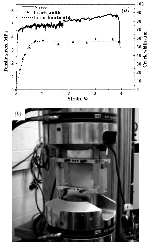
Fig. 1—(a) Typical tensile stress-strain curve and CW development of ECC; and (b) setup of uniaxial tensile loading. (Note: 1 MPa = 0.145 ksi.)
