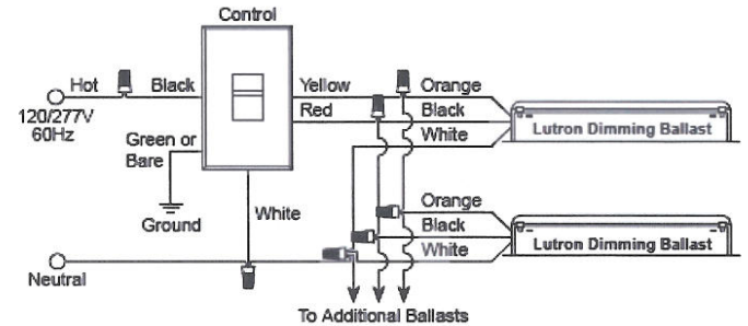
Wiring Diagram 7
