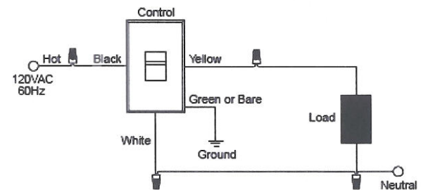
Wiring Diagram 7
