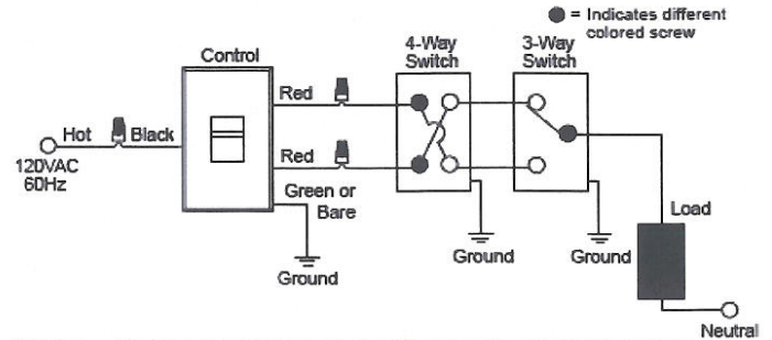
Wiring Diagram 4
