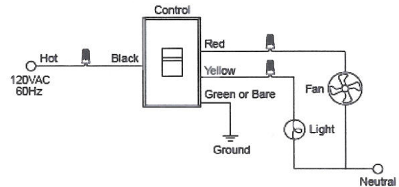
Wiring Diagram 6
