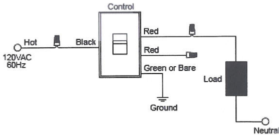
Wiring Diagram 2
