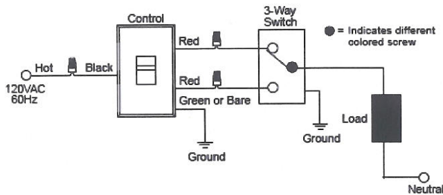
Wiring Diagram 3
