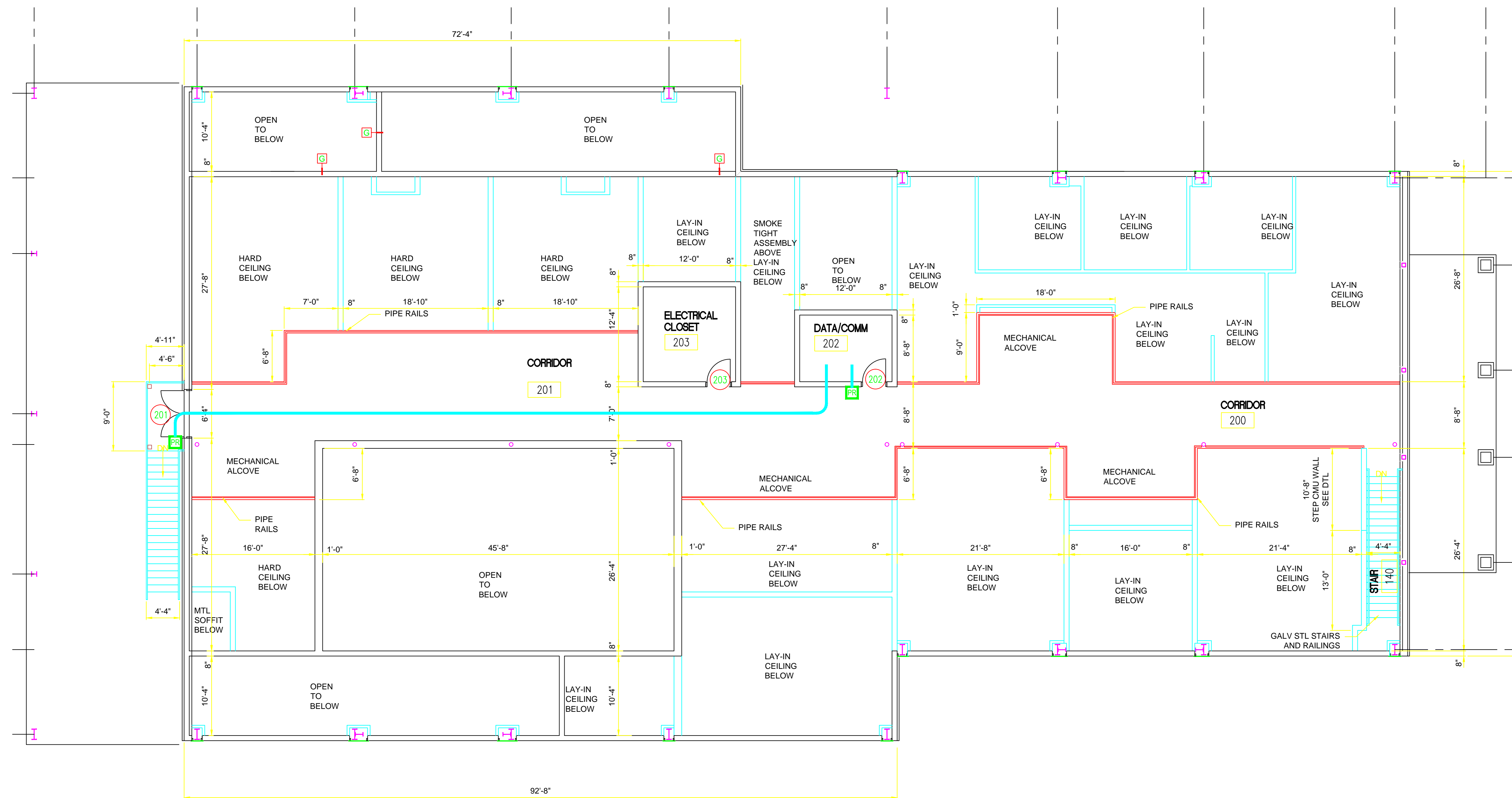
1 MEZZANINE ACCESS CONTROL PLAN SEC-1M SCALE : 1/8" = 1'-0"
