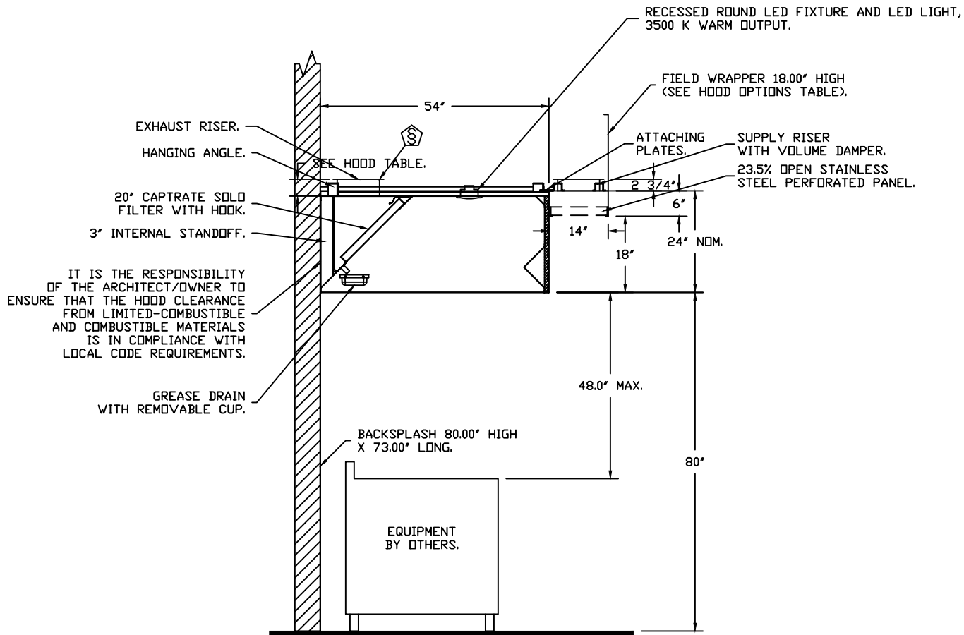
SECTION VIEW - MODEL 5424EX-2-PSP-F HOOD - #1 (KH-1)
