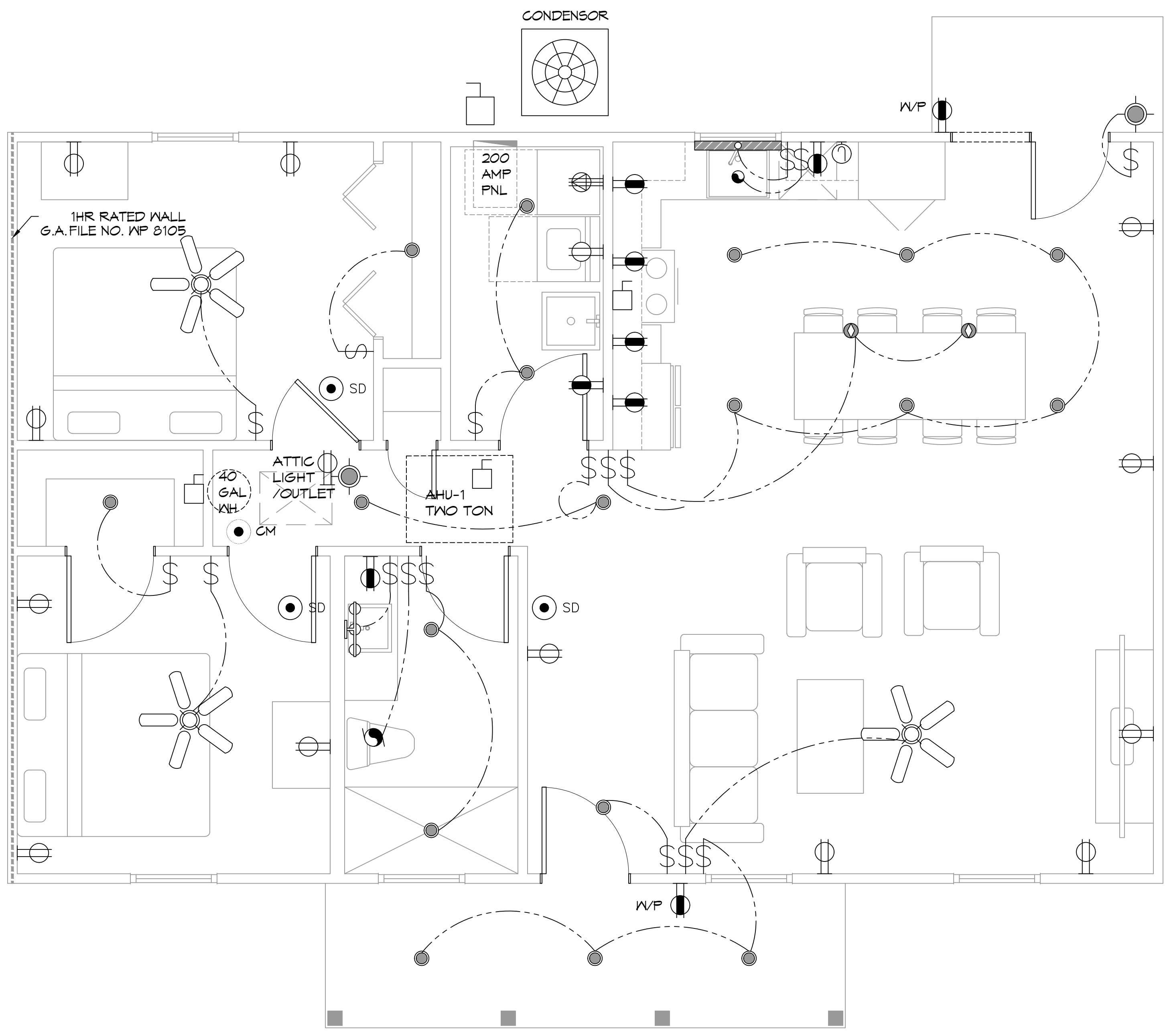
12 ELECTRICAL LIGHTING & POWER PLAN SCALE: 3/8" = 1'-0"
