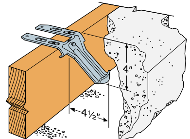
Typical MAS Installation
