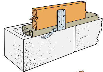
MASB Rim Joist Installation
