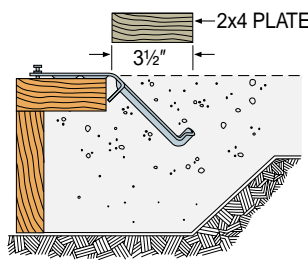
Alternate MAS Installation for Brick Ledges
