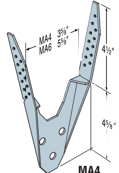
MA4 (MA6 similar)
