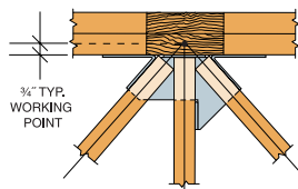
MTHM Top View Installation
