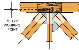
MTHM-2 Top View Installation
