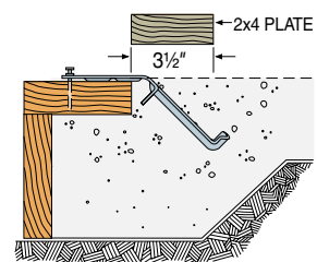
Typical MAS Installation
