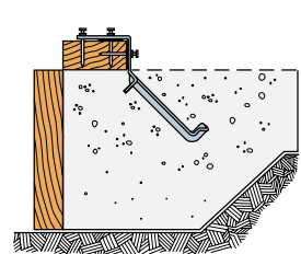
Step 2: Place mudsill on concrete and nail MAS over mudsill.
