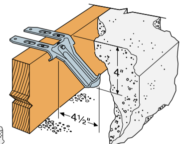
Typical MAS Installation
