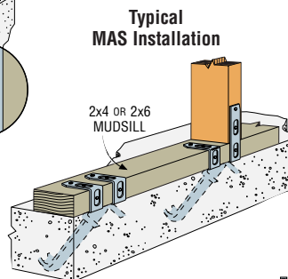
Typical MAB15 Installation in Concrete (MAB23 similar, with 15" minimum embedment)
