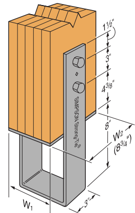
CB9 (CB5, CB7 similar) for glulam column
