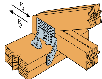
TBE6 Installed on Double 2x8 Top Plate
