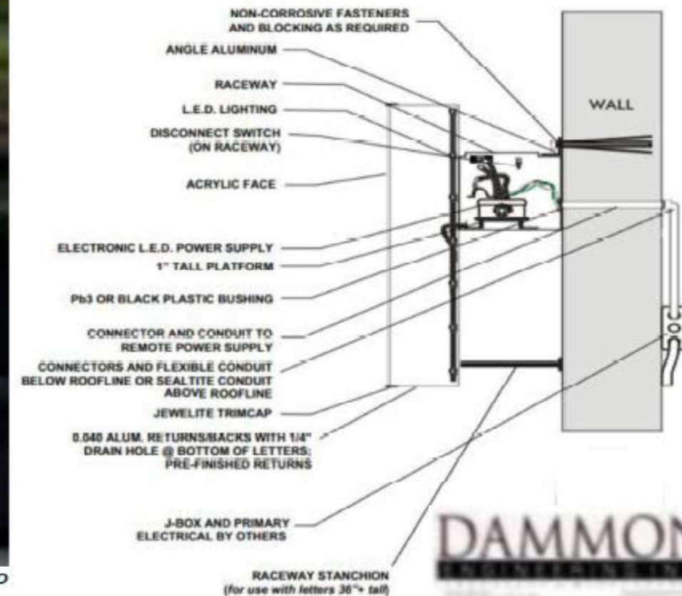
SIDE VIEW CROSS SECTION (NOT TO SCALE) NOT INTENDED FOR DETERMINING DIMENSIONS
