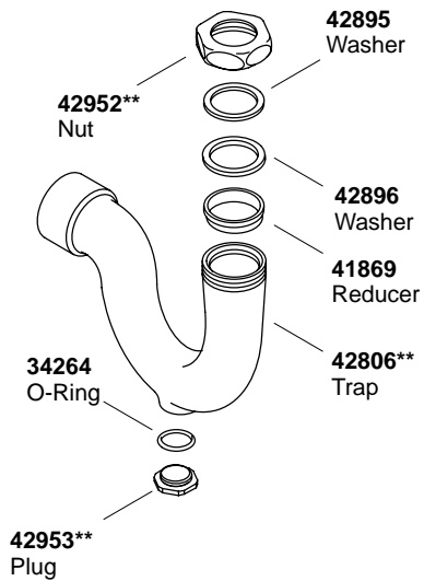
1-1/4" X 1-1/2"
