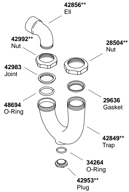
1-1/2" X 1-1/2"
