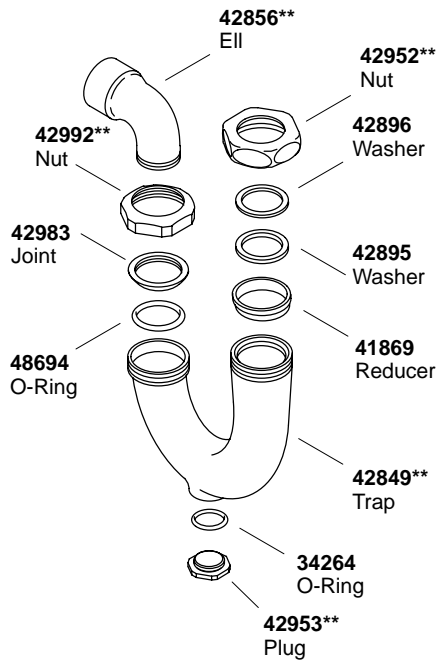
1-1/4" X 1-1/2"
