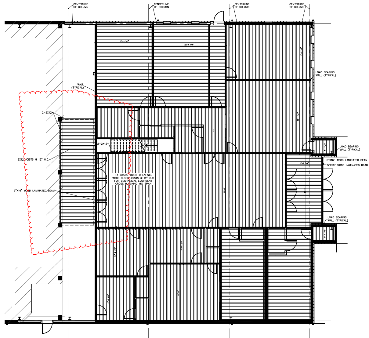
CEILING JOIST PLAN SCALE: 1/8"=1'-0"
