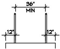
B EXTENDED SURFACE EDGE PROTECTION
