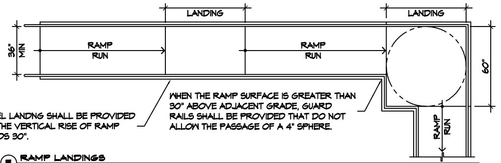
E RAMP LANDINGS
