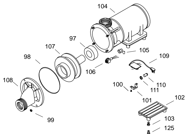
Pump w/Integral Heater 73572
