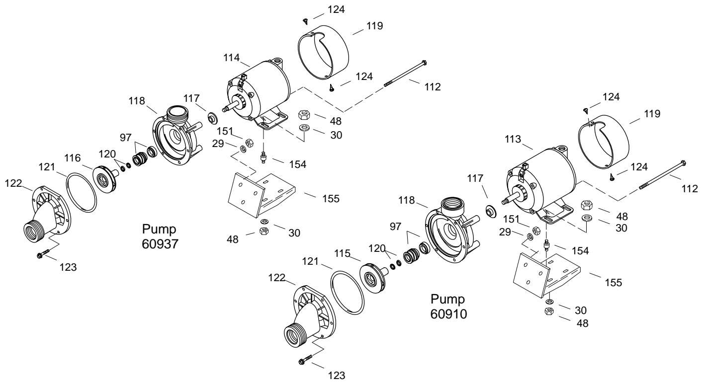
Pump w/Integral Heater 93829
