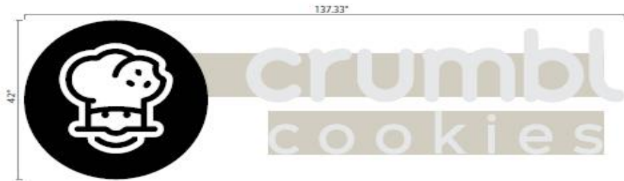
1.1 Front Lit Channel Letters on Raceway Scale : 1/2" = 1'-0"
