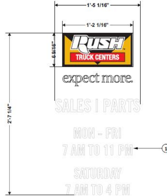
FRONT VIEW SCALE: 1 1/2"=1'-0"
