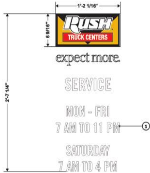
FRONT VIEW SCALE: 1 1/2"=1'-0"
