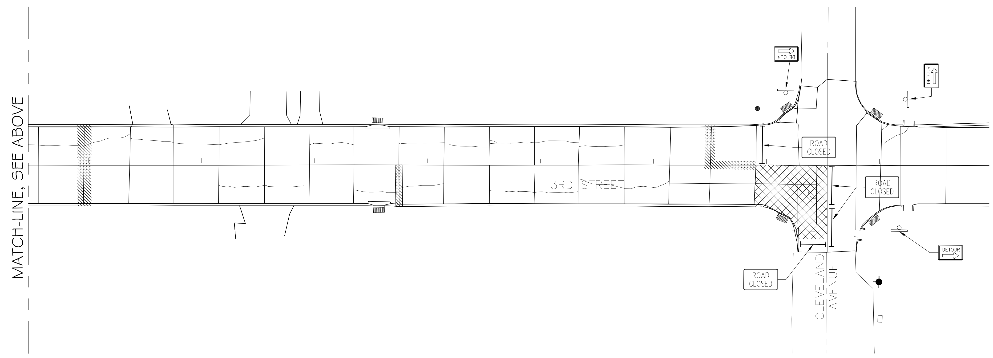
2 STREET PLAN SCALE: 1"=20'-0"
