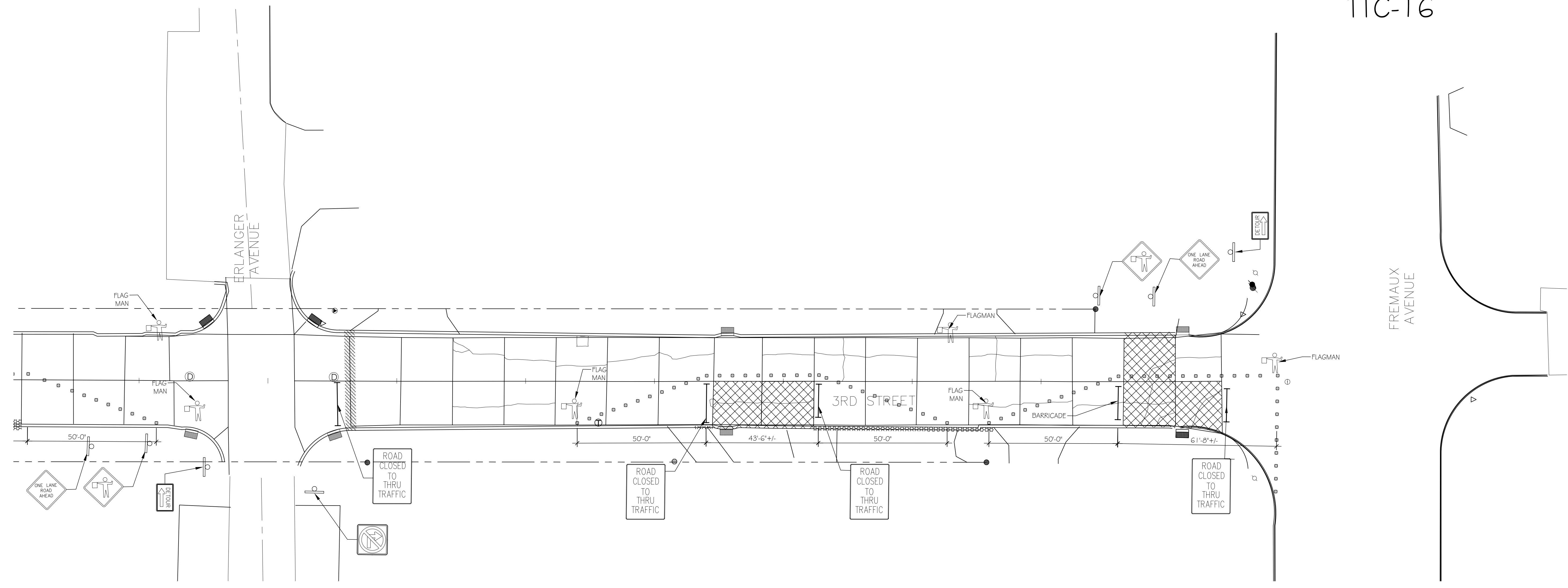
STREET PLAN SCALE: 1"=20'-0"
