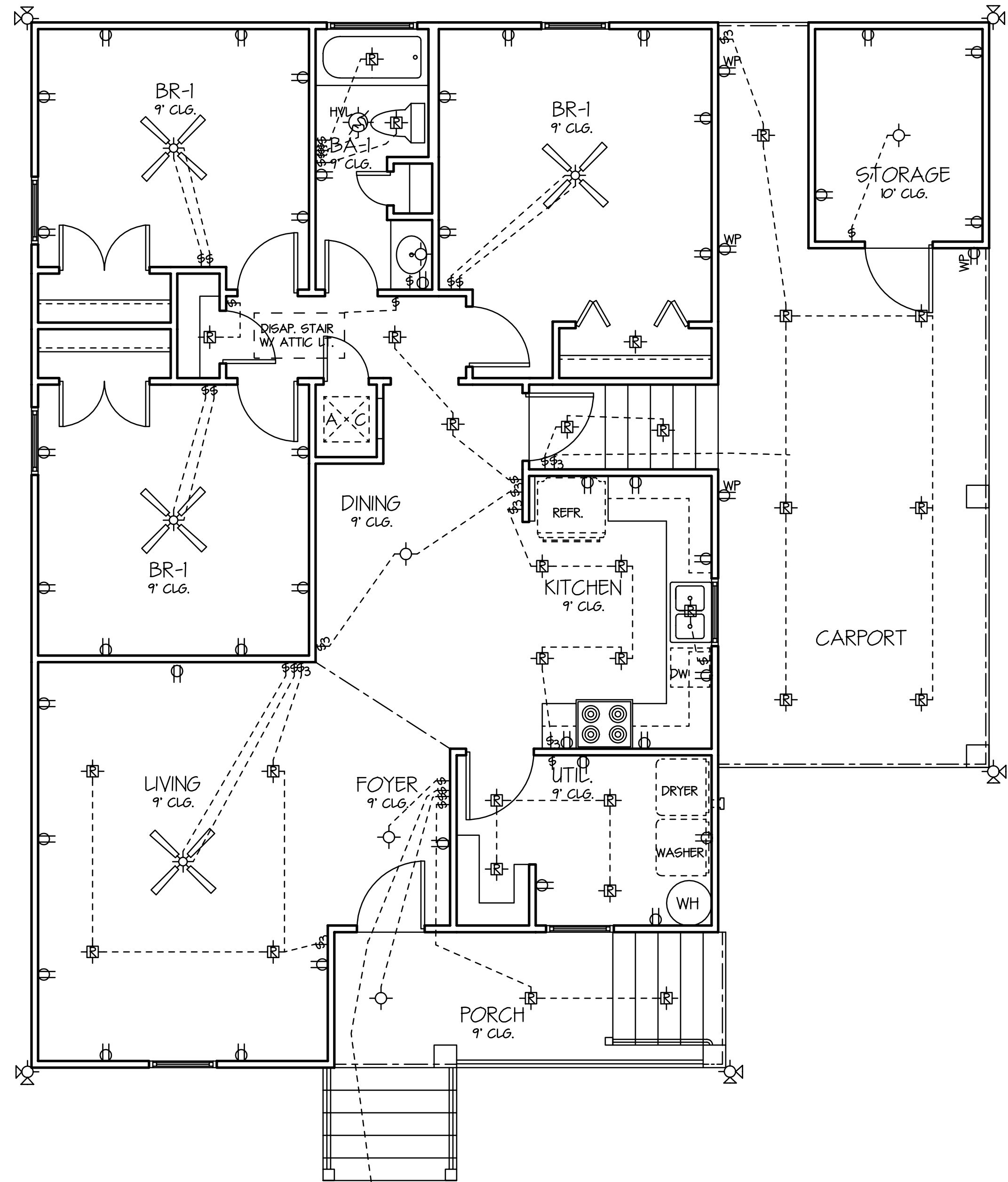
ELECTRICAL PLAN SCALE 1/4"=1'-0"
