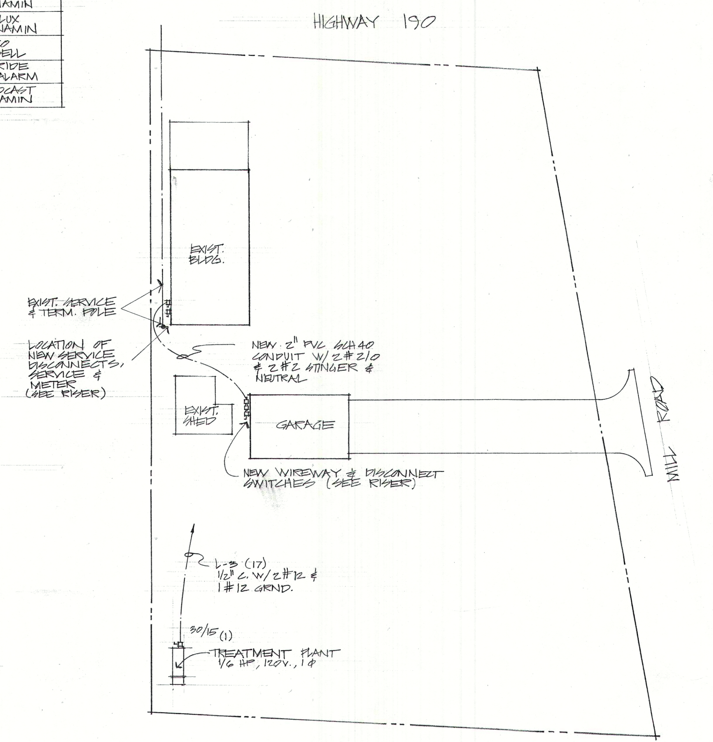
SITE PLAN
