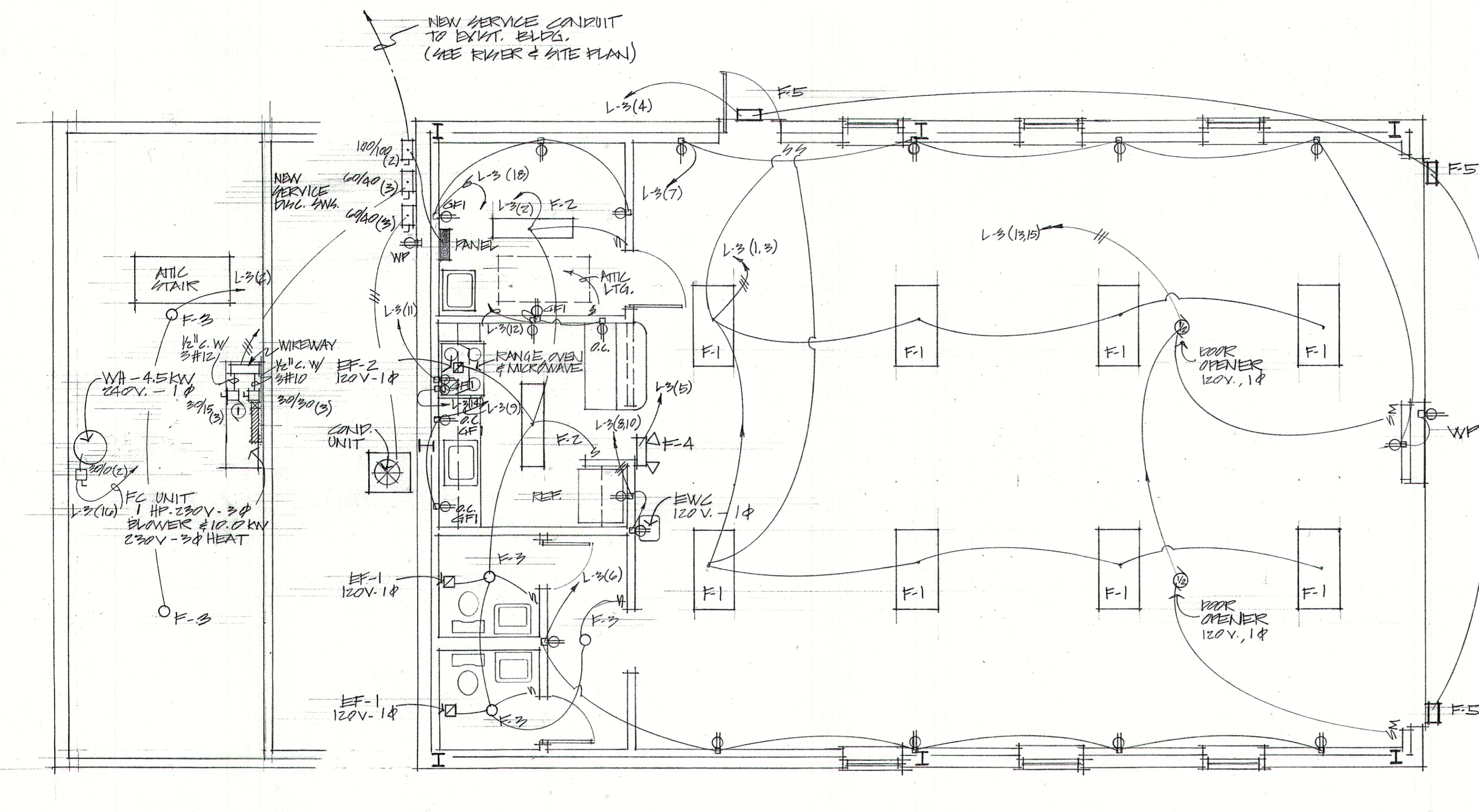
ATTIC PLAN
