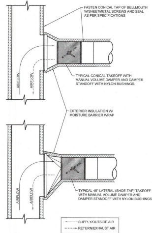
TYPICAL LOW PRESSURE RECTANGULAR TO ROUND DUCT TAKEOFF DETAIL N.T.S.
