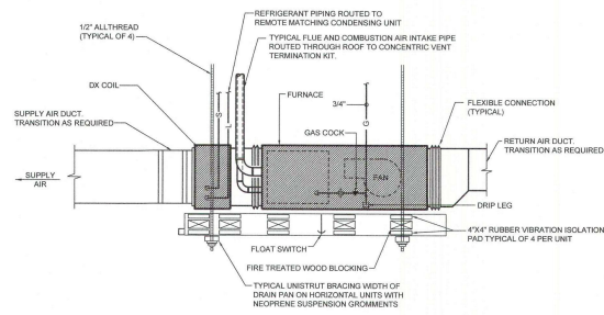
HORIZONTAL GAS FURNACE W/ DX COOLING DETAIL N.T.S.
