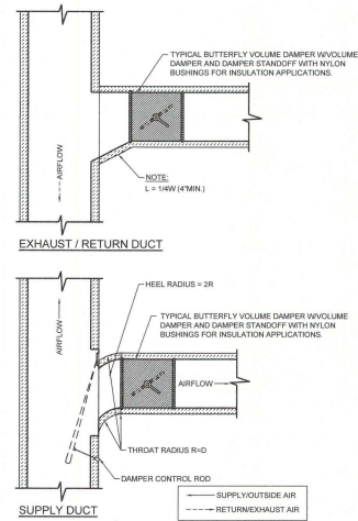
TYPICAL LOW PRESSURE RECTANGULAR TO RECTANGULAR DUCT TAKEOFF DETAIL N.T.S.
