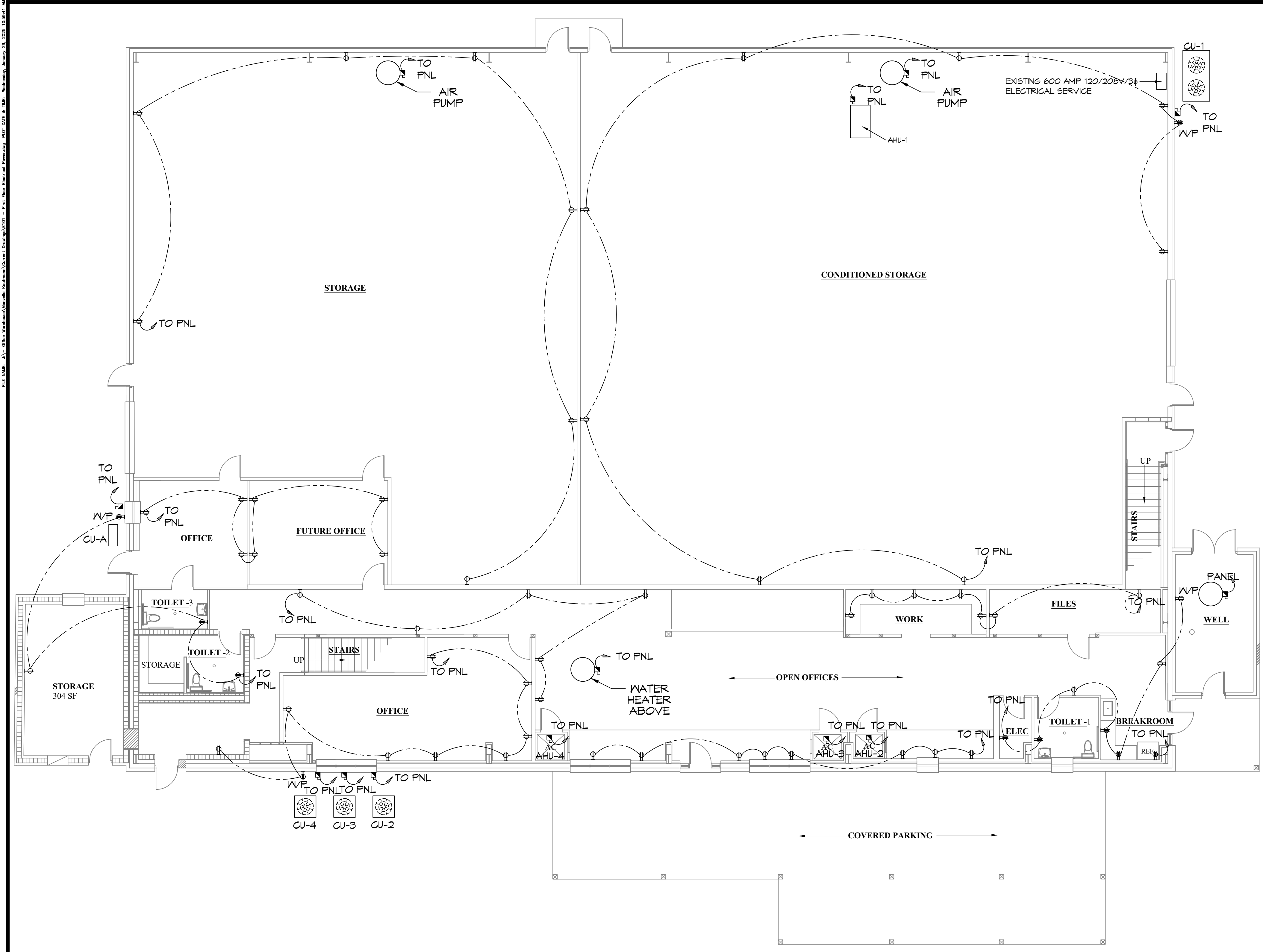
1 GROUND FLOOR POWER PLAN SCALE: 1/8"=1'-0"
