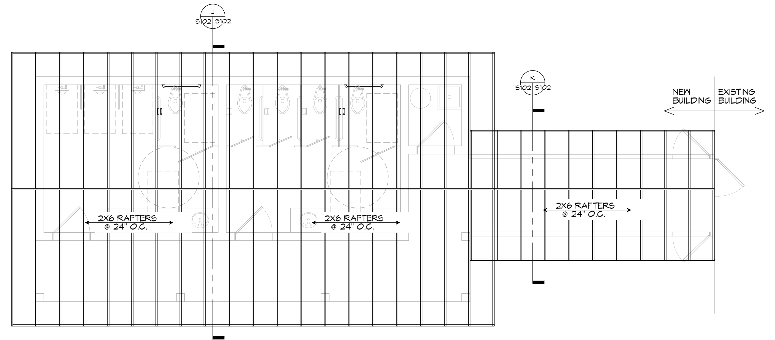
16 ROOF RAFTER FRAMING LAYOUT SCALE: 1/4" = 1'-0" RESTROOM
