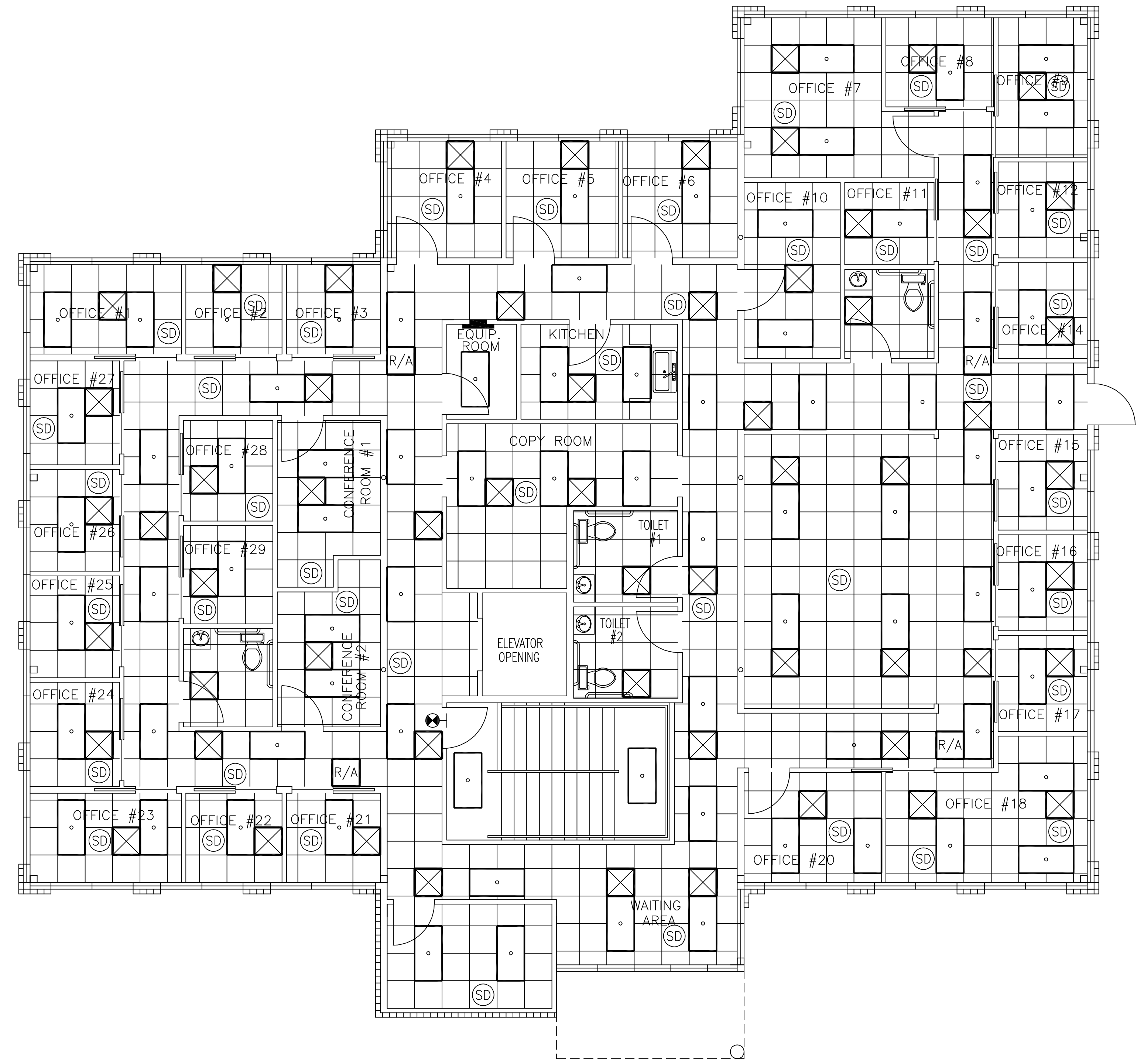
SECOND FLOOR REFLECTED CEILING PLAN SCALE: 3/16"=1'-0"
