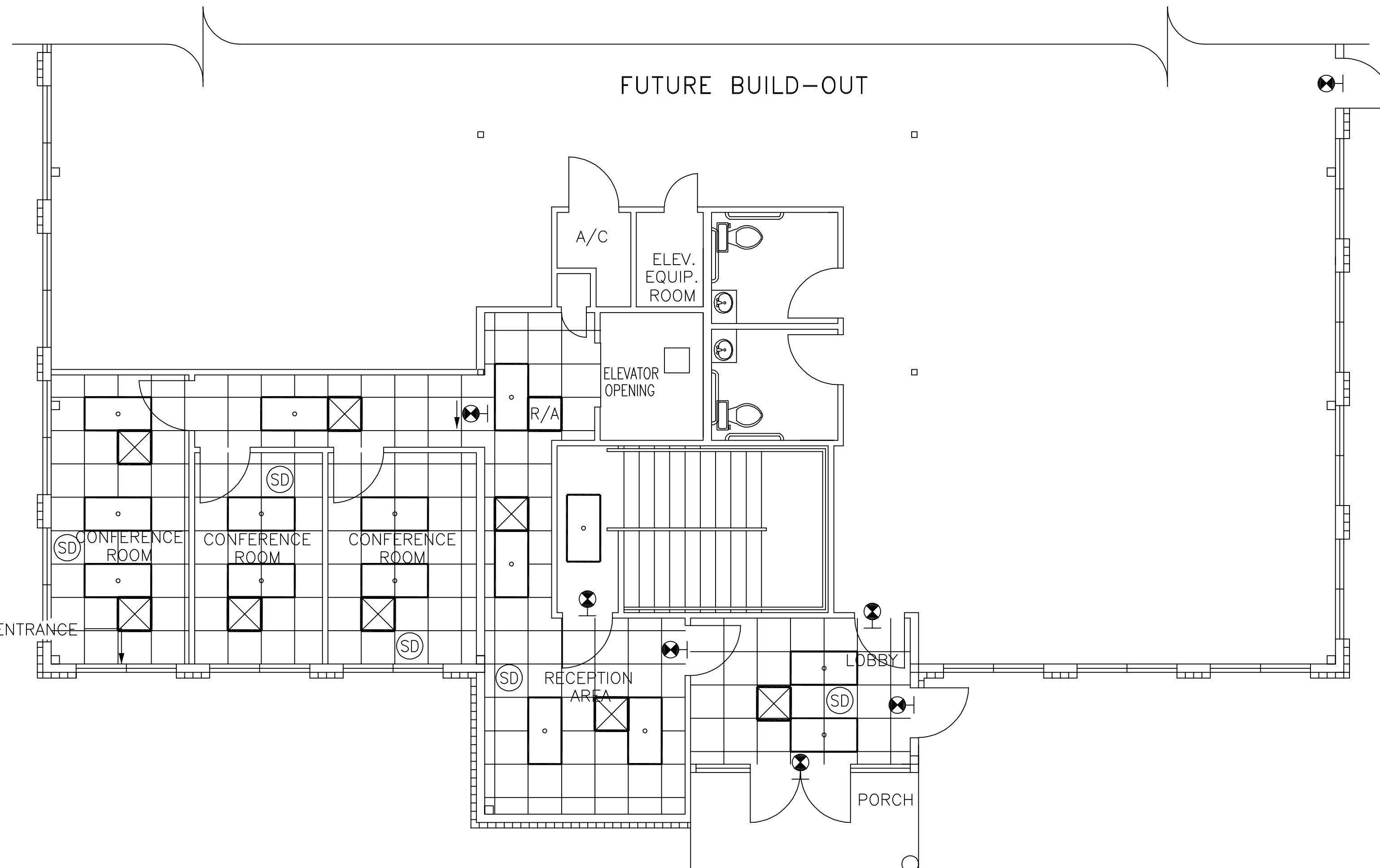
PARTIAL FIRST FLOOR REFLECTED CEILING PLAN SCALE: 3/16"=1'-0"
