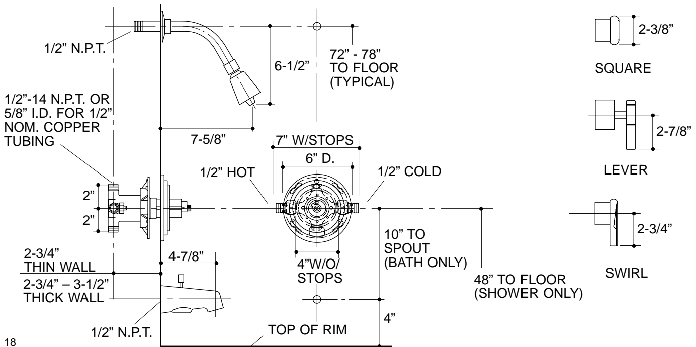
PRODUCT DIAGRAM
