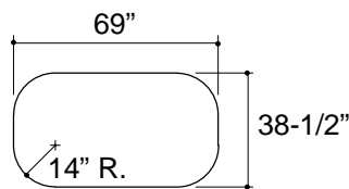
CUT-OUT DETAIL
