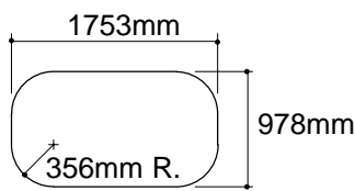
CUT-OUT DETAIL
