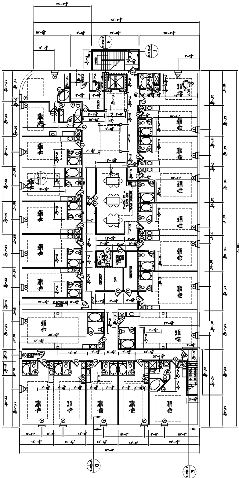
SECOND FLOOR PLAN SCALE: 1/8" = 1'-0"
