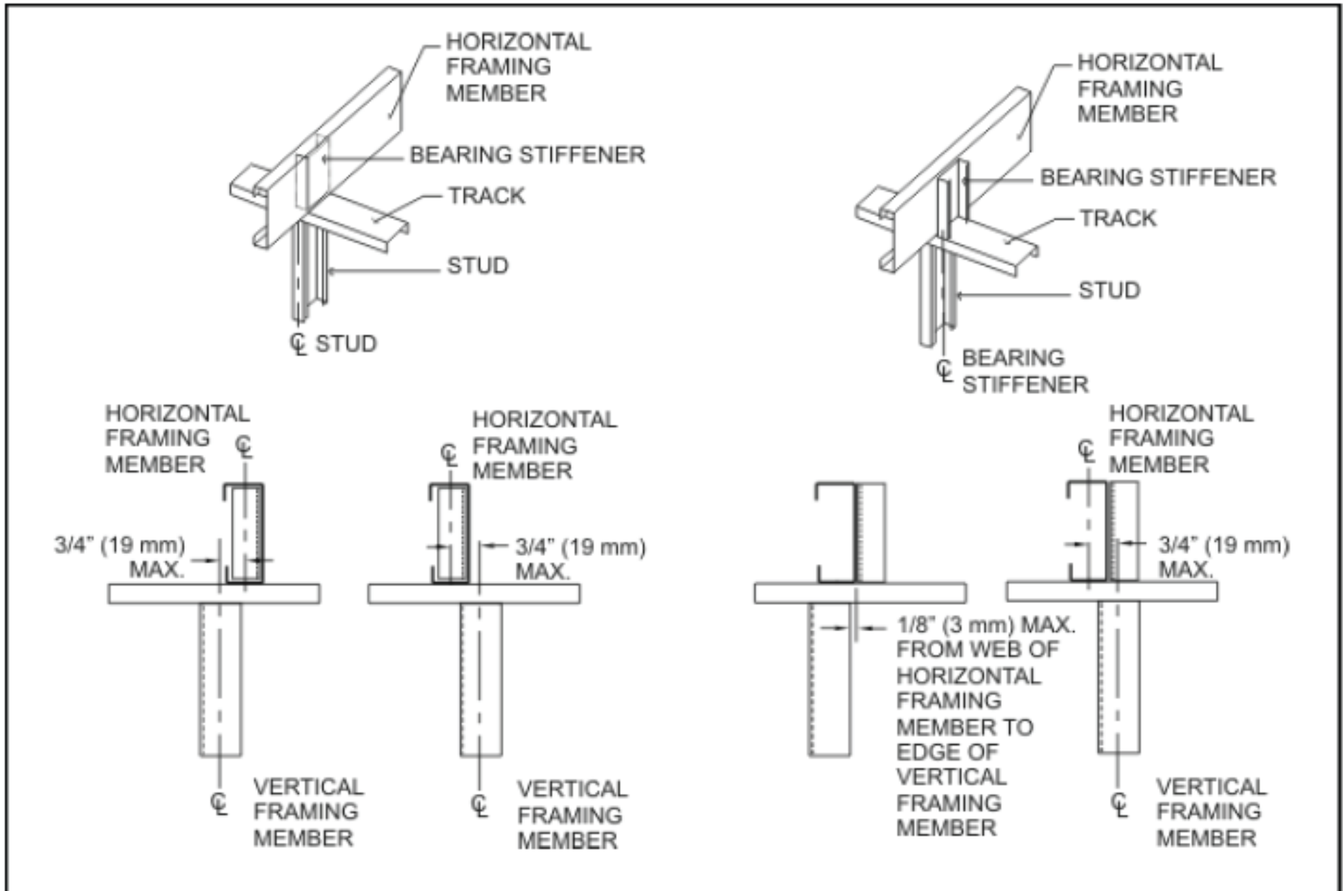
Figure B1.2.3-1 In-Line Framing
