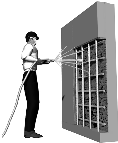
Fig. 3—Presaturate prepared surface with water.
