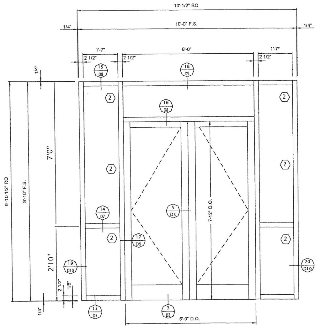
B ✓ FG-5100 IMPACT 2-1/2" X 5" 6 THUS REQ'D FINISH: BRONZE DOOR NUMBER(S): 101D, 101E, 101F, 101G, B*6, B*8, B*10, B*12, B*14
