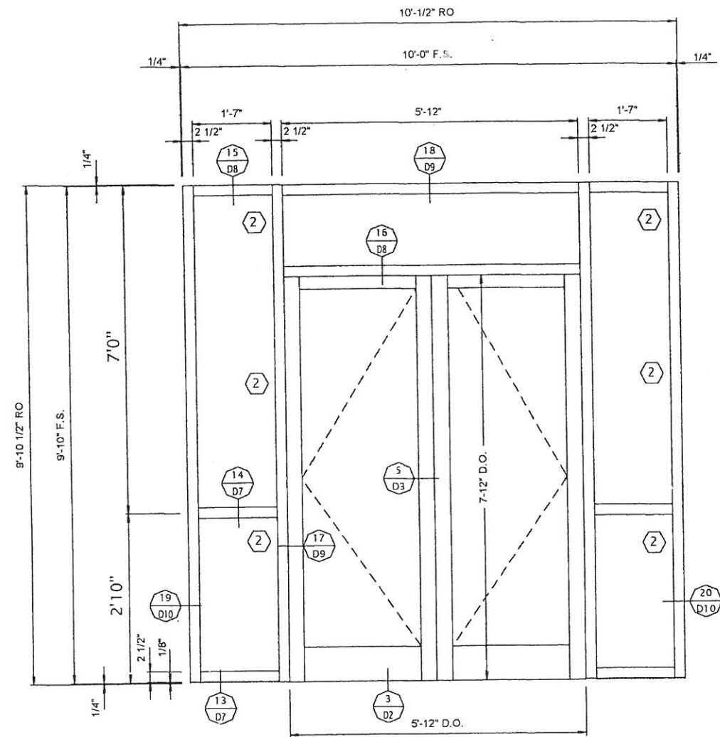
A ✓ FG-5100 IMPACT 2-1/2" X 5" 1 THUS REQ'D FINISH: BRONZE DOOR NUMBER(S): 101A
