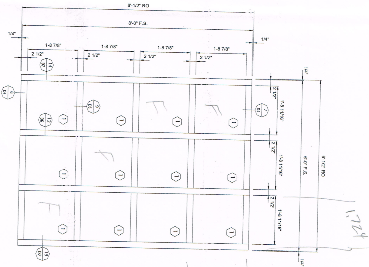
HR-251 IMPACT CURTAINWALL 2-1/2" X 7 1/2" 2 THUS REQ'D FINISH: CLEAR
