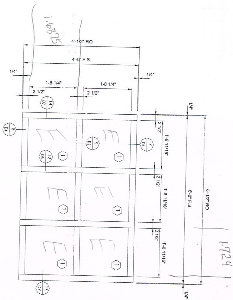
HR-251 IMPACT CURTAINWALL 2-1/2" X 7 1/2" 3 THUS REQ'D FINISH: CLEAR
