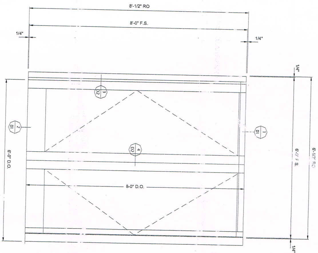
HR-251 IMPACT CURTAIN WALL 2-1/2" X 7 1/2" FINISH CLEAR DOOR NUMBER(S): 1 A*4
