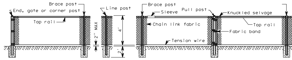
CHAIN LINK FENCE TYPE 6
