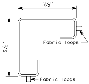
END, CORNER AND PULL POST
