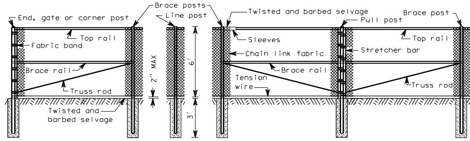
CHAIN LINK FENCE TYPE 1
