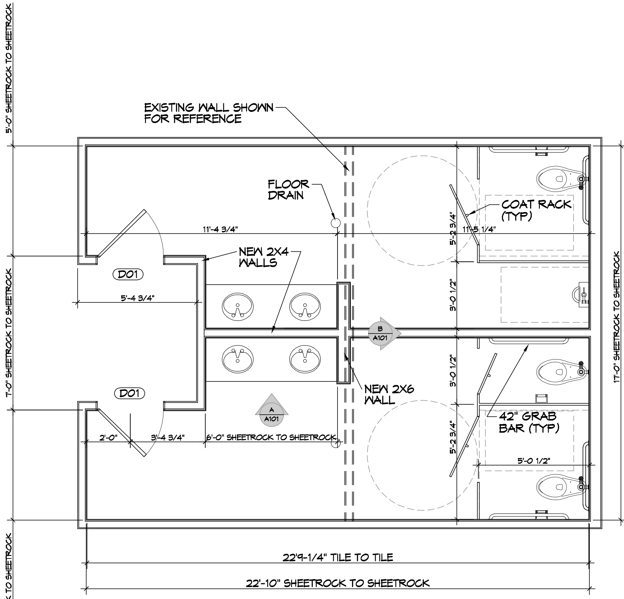
1 FLOOR PLAN SCALE: 3/8" = 1'-0"
