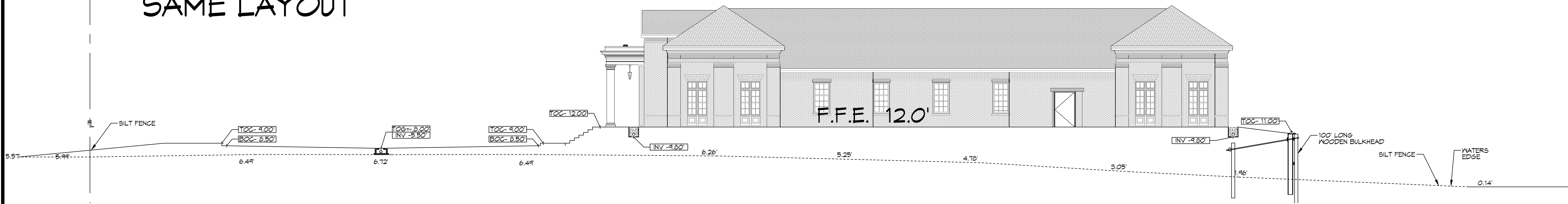
B CROSS SECTION C5 SCALE: 1"=10'-0"
