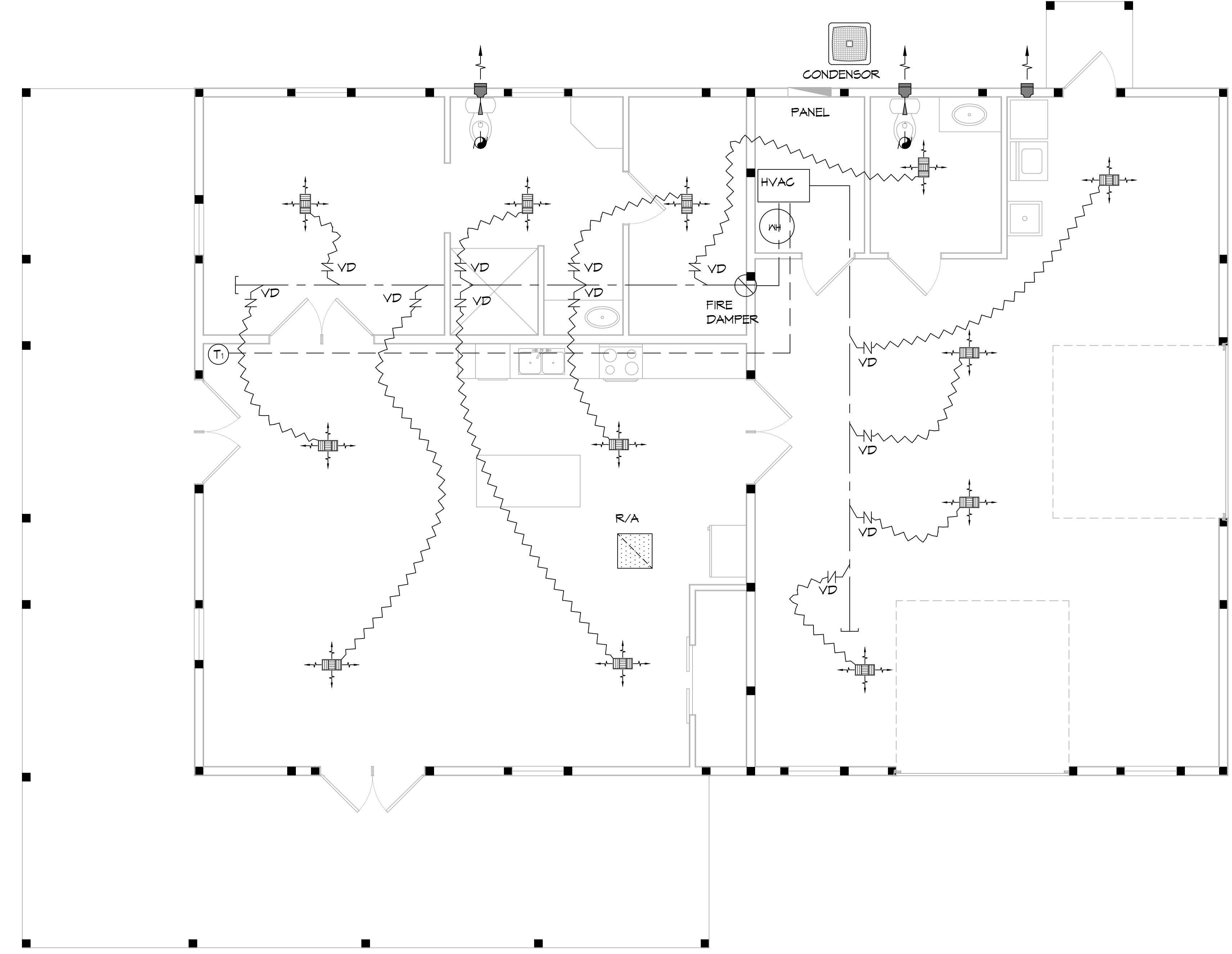
4 MECHANICAL PLAN SCALE: 1/4" = 1'-0"
