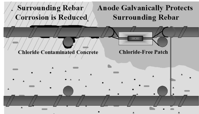
Fig. 2—Chloride-accelerated corrosion.
