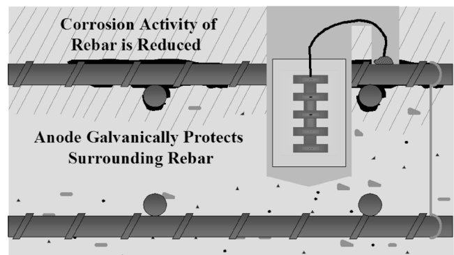
Fig. 3—Chloride-accelerated corrosion.
