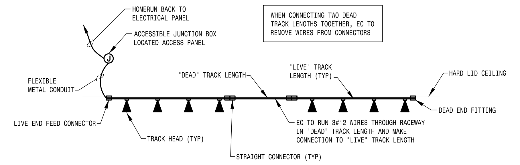
2 TRACK WIRING DIAGRAM (HARD CEILING) E1.1.0 SCALE: NONE
