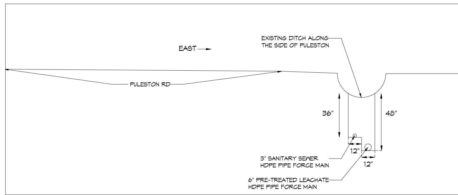
D M101B/M101B 1/4" = 1'-0"
