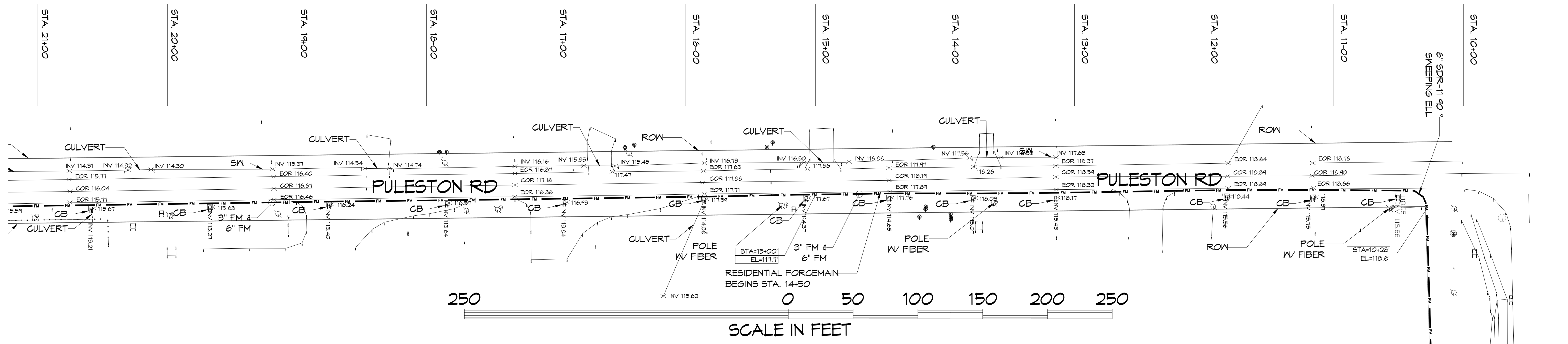
3 M101B/M101 1" = 40' PRE-TREATED LEACHATE AND SEWER FORCE MAINS PARTIAL SITE PLAN
