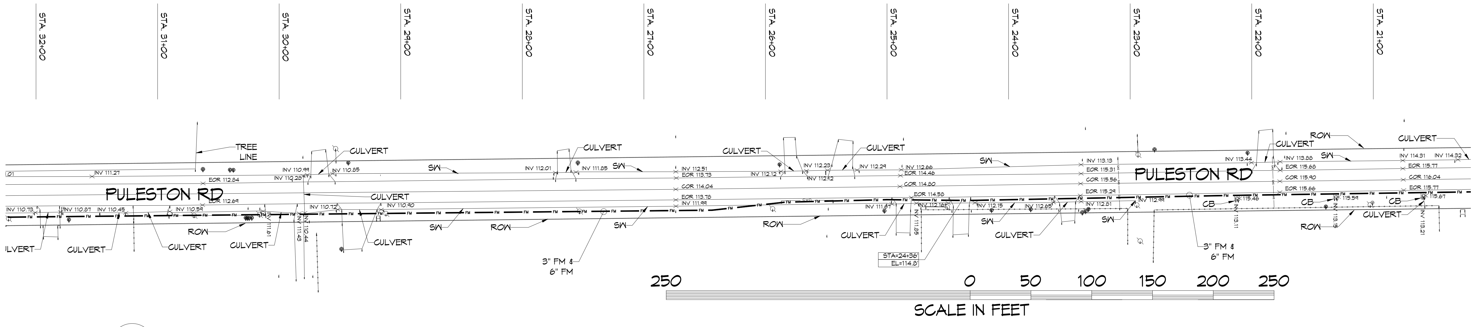
4 M101B/M101 1" = 40' PRE-TREATED LEACHATE AND SEWER FORCE MAINS PARTIAL SITE PLAN
