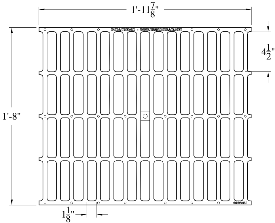
20B24DI DUCTILE IRON GRATE
