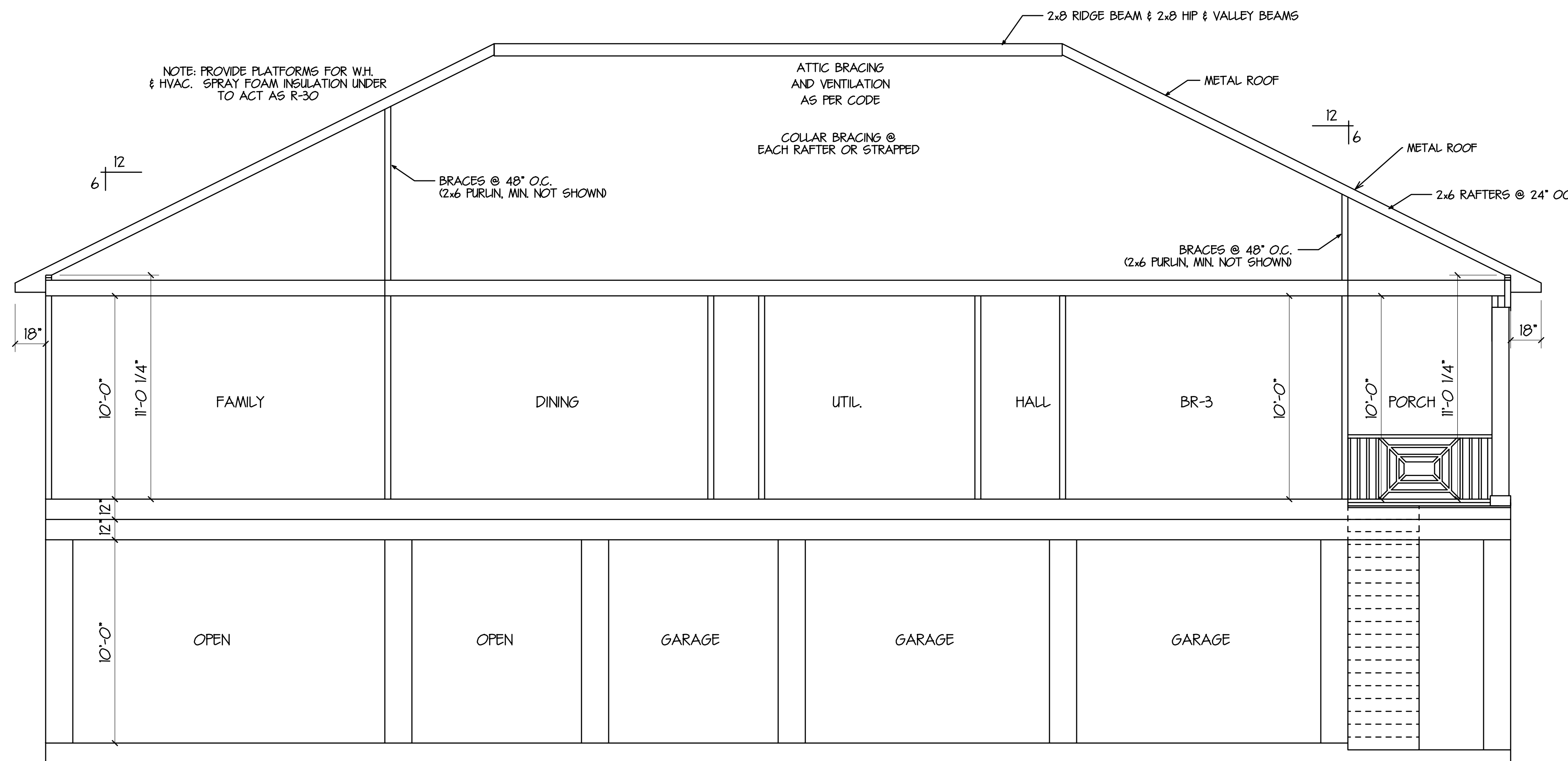
TYPICAL CROSS SECTION SCALE 1/4" = 1'-0" SEE PLANS BY ENGINEER FOR FOUNDATION DESIGN AND SIZE AND SPACING OF GILL, FLOOR JOIST AND PEIRS.
