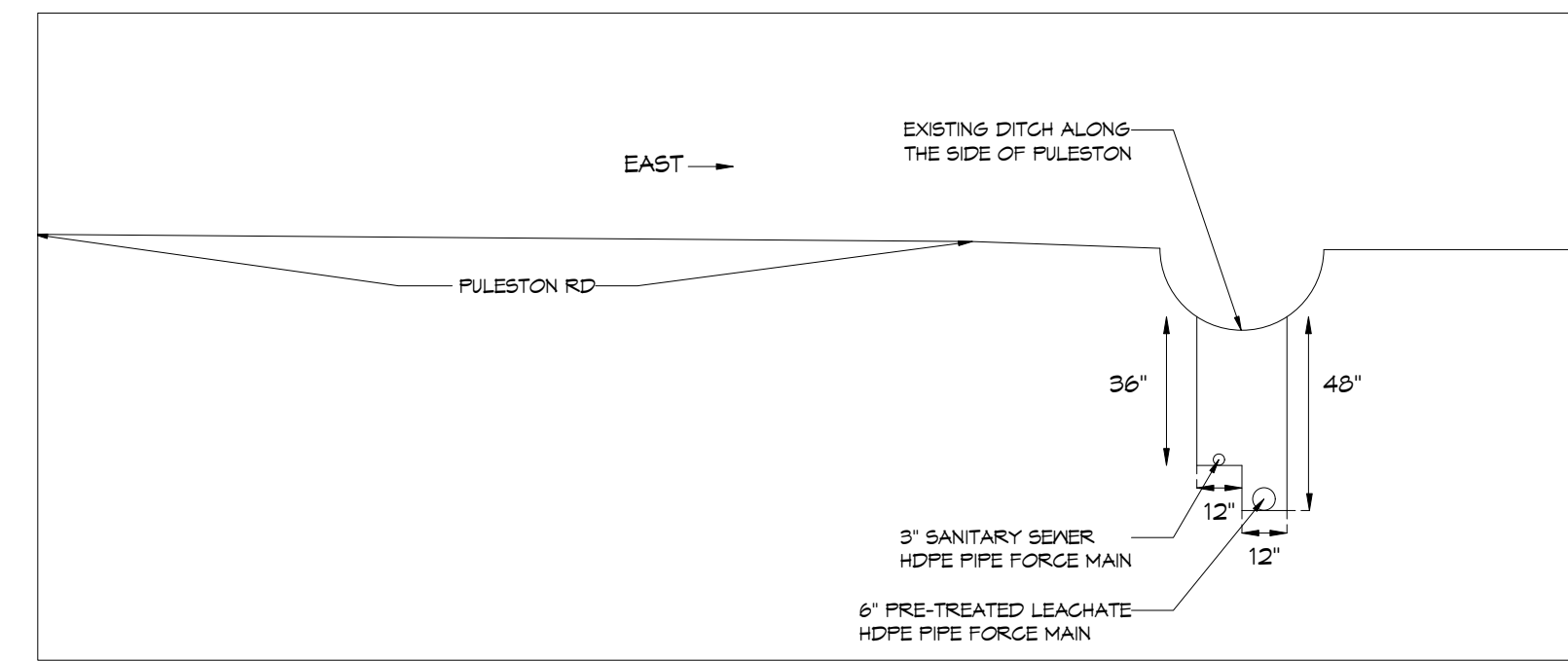
D M101B/M101B 1/4" = 1'-0"
